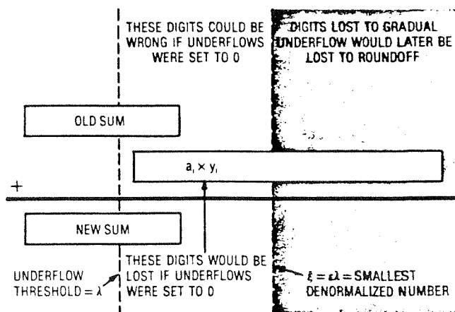
Figure 10. The effect of gradual underflow and Store 0 on small sums in one step of the cited program loop.
