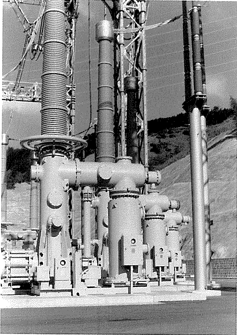
Picture of MOSA for 500kV GIS used in Japanese electric company in 1979
