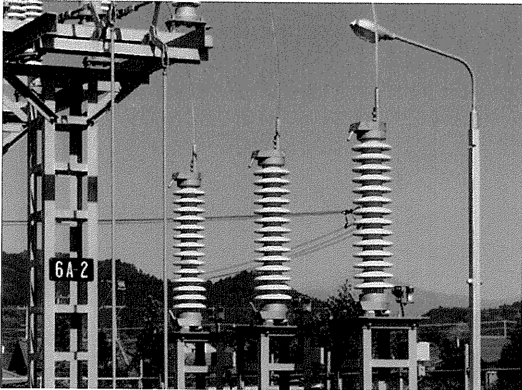
Picture of MOSA for 66kV system used in Japanese electric company in 1975
