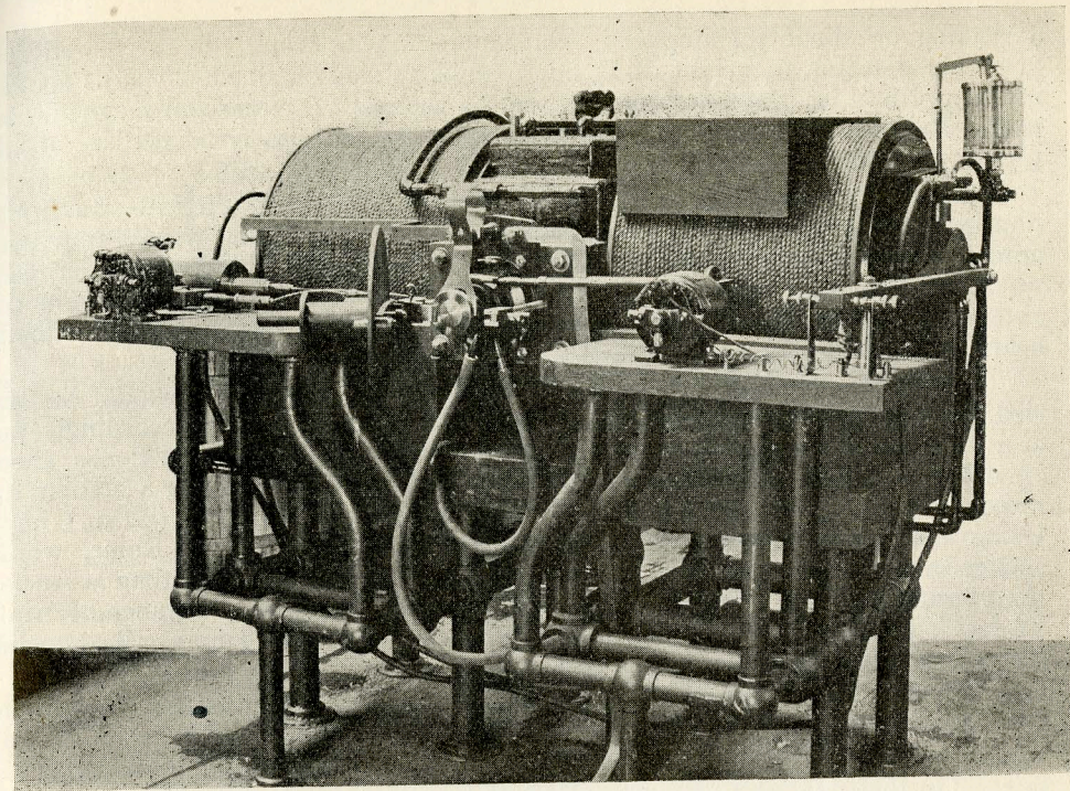
Figure 25b—Federal Telegraph Company 100 k.w. Poulsen arc at Darien
