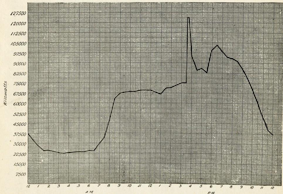
Figure 4.—An example of a load curve of a lighting central station for a March day (1911) during which a severe unexpected storm took place at 3:30 P. M. But for the abnormal peak occurring because of this storm, the curve would be similar to that of Figure 3.
