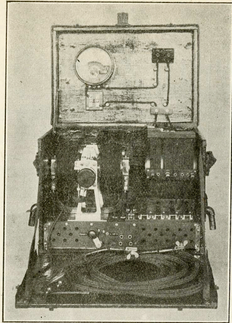
Figure 15—Berliner-Poulsen arc for portable stations
