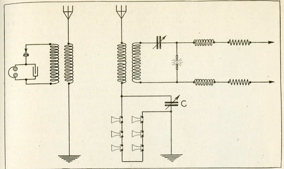
Figure 17—Poulsen radiophone transmitter and receiver
