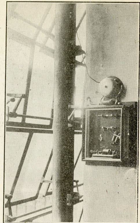
Receiving apparatus of the wireless storm detector
