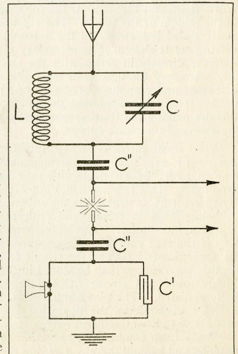
Figure 18—Flywheel Poulsen arc circuit for radio telephony
