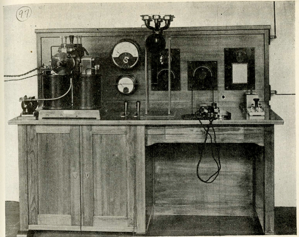
Figure 23—Berliner-Poulsen arc ship radiophone station
