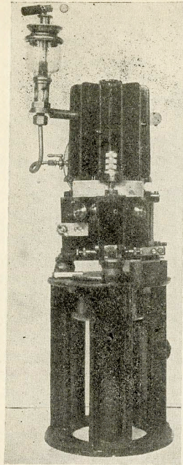
Figure 19—Lorenz-Poulsen arc for radio telephony
