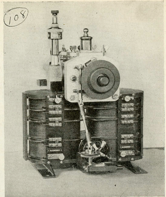
Figure 21—3 k.w. Berliner-Poulsen arc
